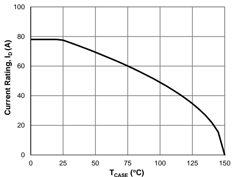
Figure 7: Current De-rating
