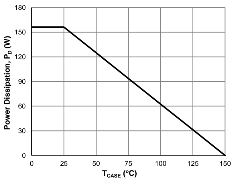
Figure 8: Power De-rating
