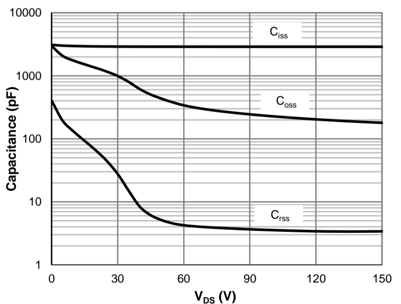
Figure 6: Capacitance Characteristics
